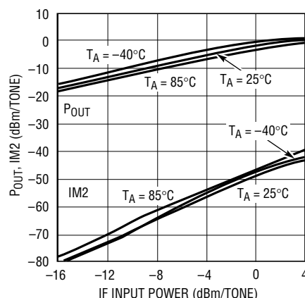
RF Output Power and Output IM2 vs IF Input Power (Two Input Tones)
