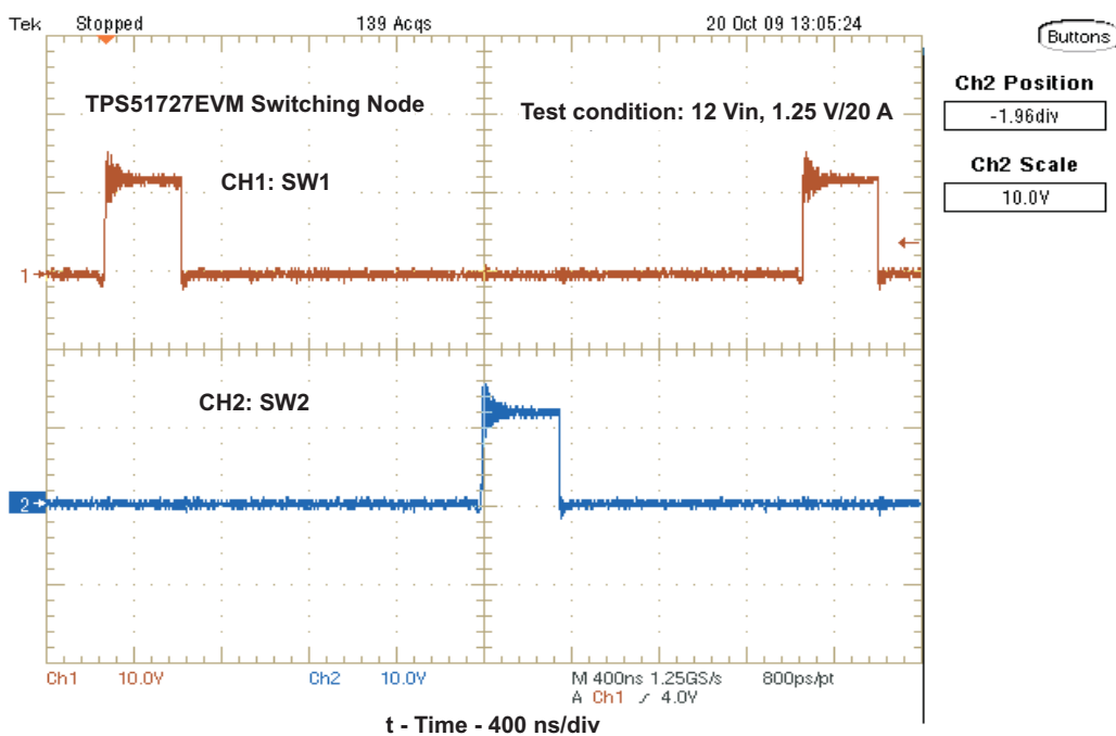
Figure 11. Switching Node
