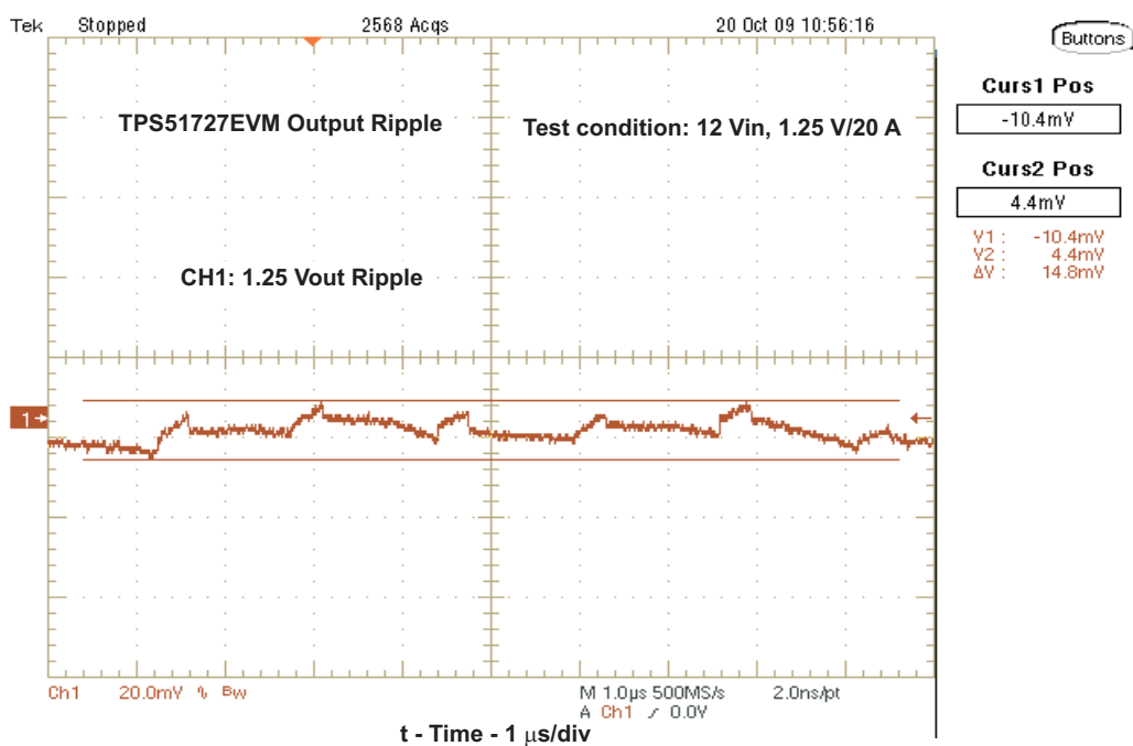
Figure 10. TPS51727EVM Output Ripple
