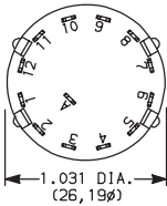
TERM. NOS. MOLDED ON HOUSING
