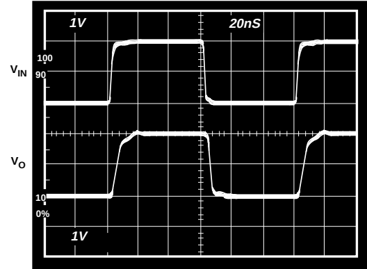
Figure 20. Small Signal Pulse Response, Gain = +1, R_F = 1\text{ k}\Omega , R_L = 150\text{ }\Omega , V_S = \pm 15\text{ V}
