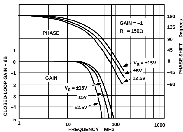
Figure 33. Closed-Loop Gain and Phase vs. Frequency G = -1 , R_L = 150 \Omega , R_F = 681 \Omega for \pm 15 \text{ V} , 620 \Omega for \pm 5 \text{ V} and \pm 2.5 \text{ V}
