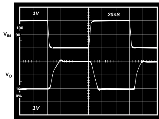
Figure 32. Small Signal Pulse Response, Gain = -1, R_F = 681 \Omega , R_L = 150 \Omega , V_S = \pm 5 \text{ V}
