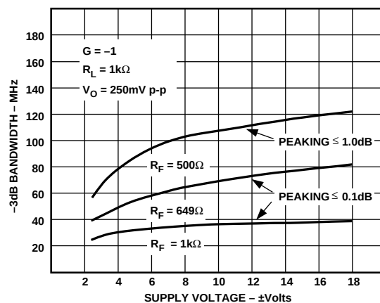
Figure 36. -3 dB Bandwidth vs. Supply Voltage, Gain = -1, R_L = 1 \text{ k}\Omega
