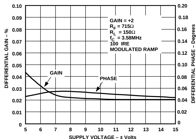
Figure 49. Differential Gain and Phase vs. Supply Voltage
