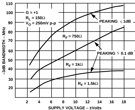
Figure 23. Bandwidth vs. Supply Voltage, Gain = +1, R_L = 150\text{ }\Omega
