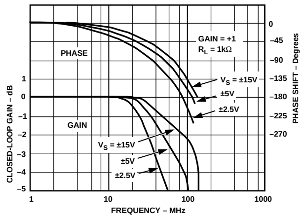
Figure 22. Closed-Loop Gain and Phase vs. Frequency, G = +1 , R_F = 1\text{ k}\Omega for \pm 15\text{ V} , 910\text{ }\Omega for \pm 5\text{ V} and \pm 2.5\text{ V}
