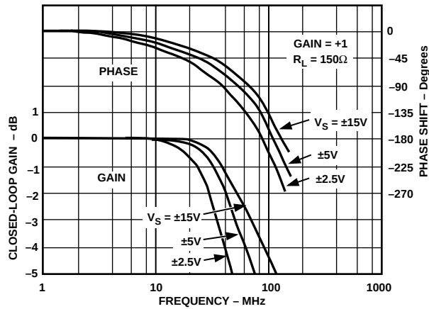
Figure 21. Closed-Loop Gain and Phase vs. Frequency, G = +1 , R_F = 1\text{ k}\Omega for \pm 15\text{ V} , 910\text{ }\Omega for \pm 5\text{ V} and \pm 2.5\text{ V}
