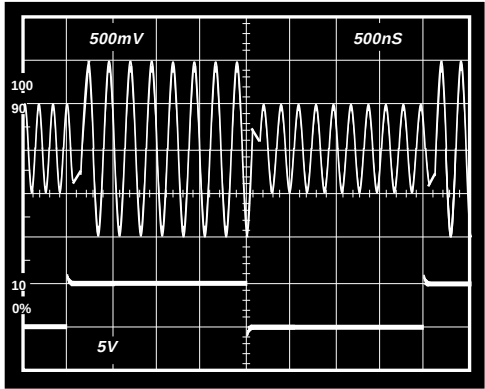
Figure 52. Channel Switching Time for the 2:1 Mux
