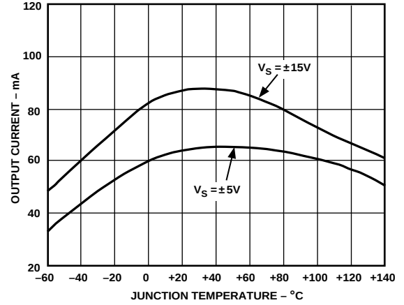
Figure 8. Linear Output Current vs. Temperature
