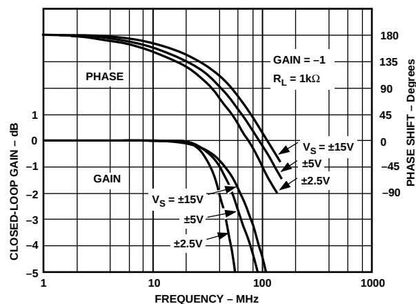
Figure 34. Closed-Loop Gain and Phase vs. Frequency, G = -1 , R_L = 1 \text{ k}\Omega , R_F = 681 \Omega for V_S = \pm 15 \text{ V} , 620 \Omega for \pm 5 \text{ V} and \pm 2.5 \text{ V}
