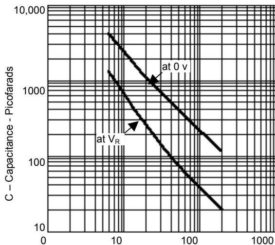
V_Z – Zener Voltage – Volts FIGURE 3 – Capacitance vs Zener Voltage
