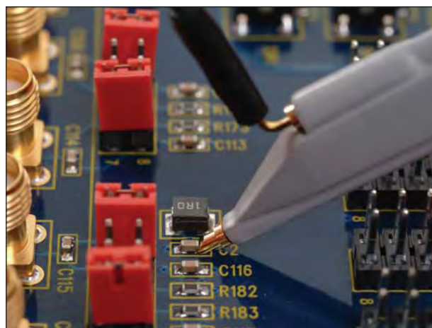
Probe directly on surface mount components, like resistors or capacitors, with the Discrete SMD Tip. Use this tip with any of the ground leads, like the flexible Long Right-angle Lead shown here.
