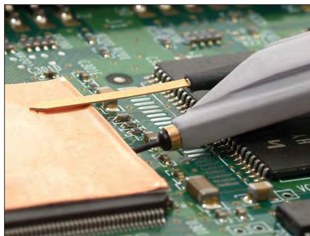
The Ground Blade and Copper Pad provide the shortest ground loop for excellent signal fidelity when probing an IC. Use them with the insulated IC Lead Tip to prevent shorting between test points.
