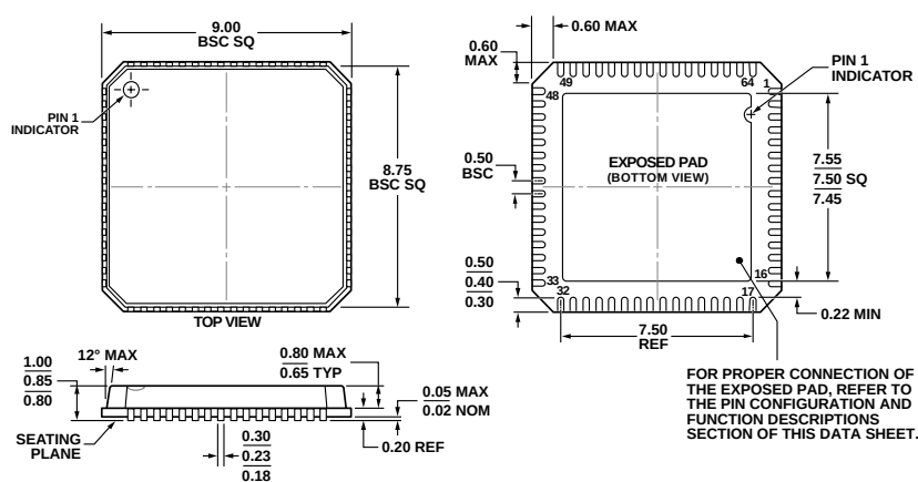
COMPLIANT TO JEDEC STANDARDS MO-220-VMMD-4 Figure 101. 64-Lead Lead Frame Chip Scale Package [LFCSP_VQ] 9 mm × 9 mm Body, Very Thin Quad (CP-64-6) Dimensions shown in millimeters
