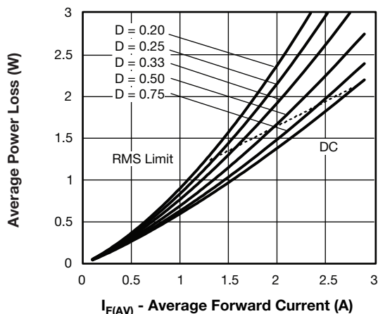
I_{F(AV)} - Average Forward Current (A) Fig. 5 - Maximum Average Forward Dissipation vs. Average Forward Current
