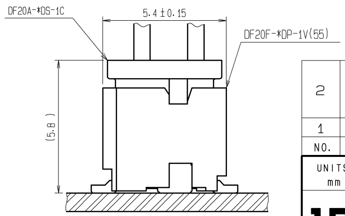
APPLICATION DIAGRAM(FREE)
