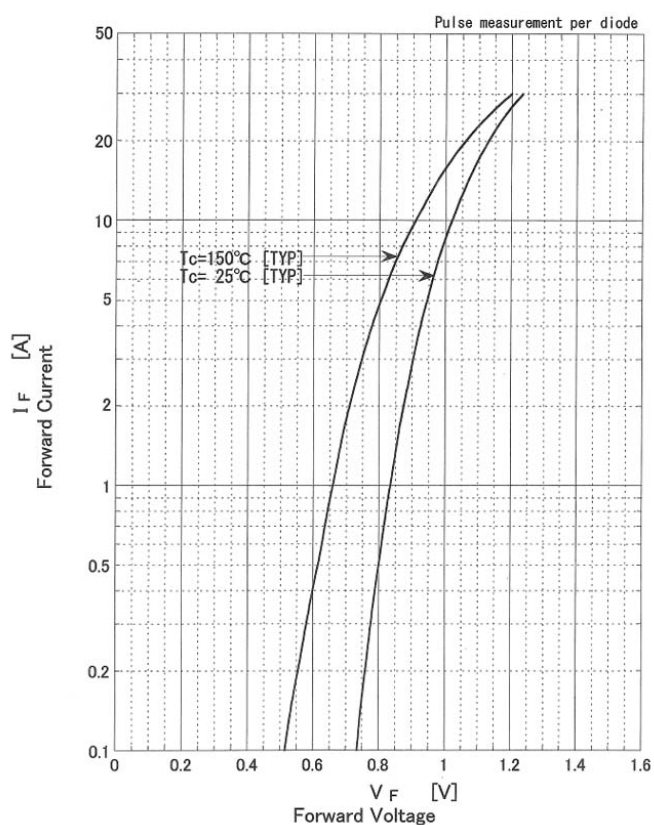
Forward Voltage
