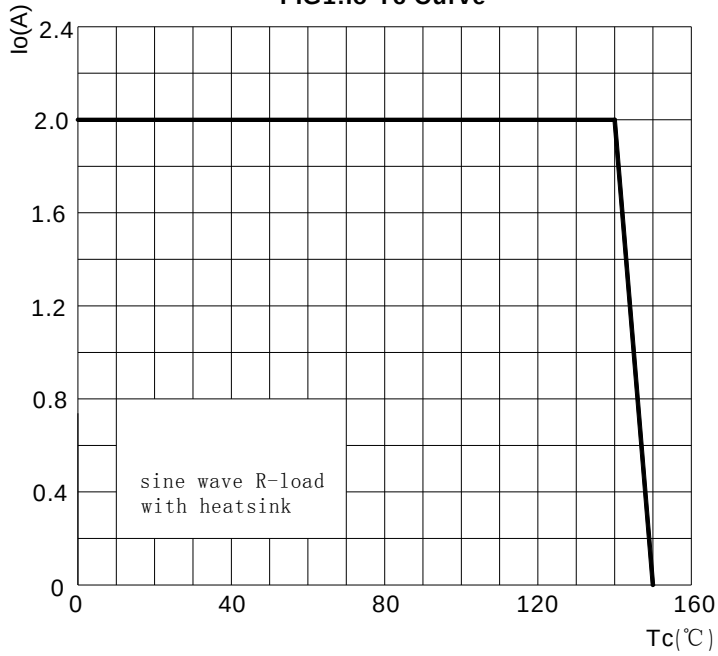
FIG1:Io-Tc Curve
