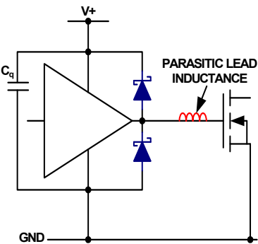
FIGURE 15. SUGGESTED CONFIGURATION FOR DRIVING INDUCTIVE LOADS
