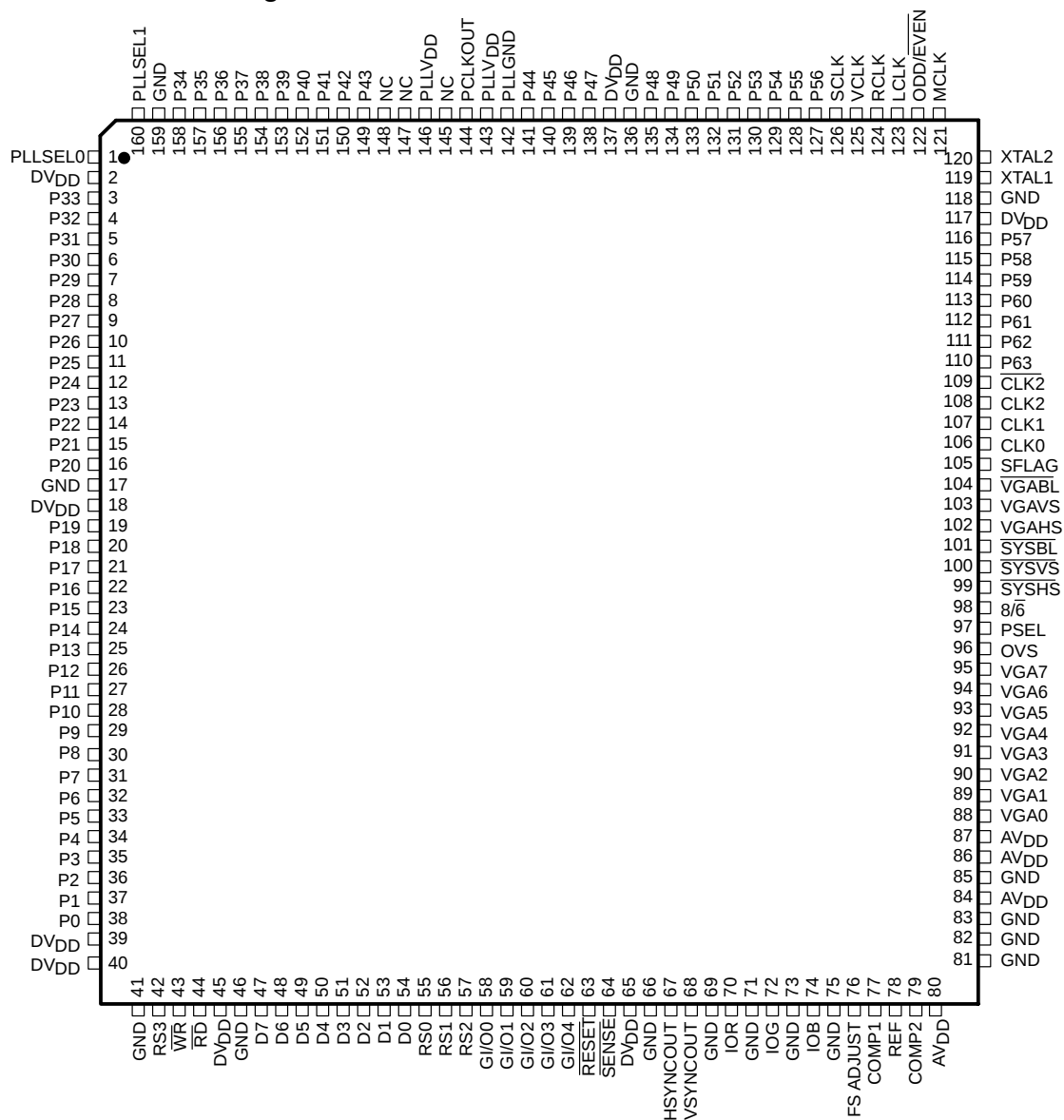
Figure 1–2. Terminal Assignments
