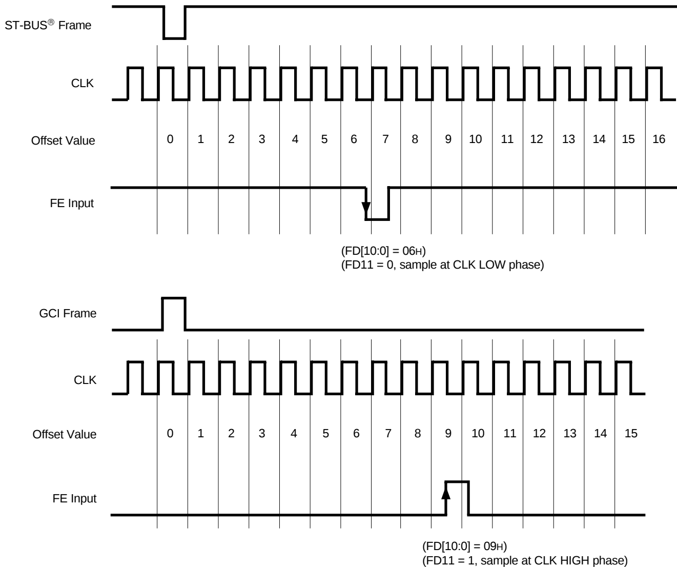
Figure 1. Example for Frame Alignment Measurement
