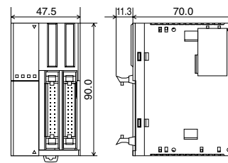
FC4A-D40K3, FC4A-D40S3
