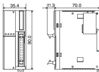
FC4A-D20K3, FC4A-D20S3
