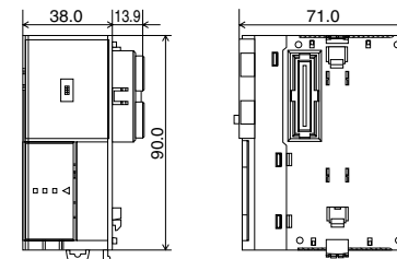
FC4A-HPH1
