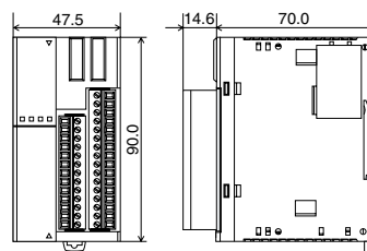
FC4A-D20RK1, FC4A-D20RS1
