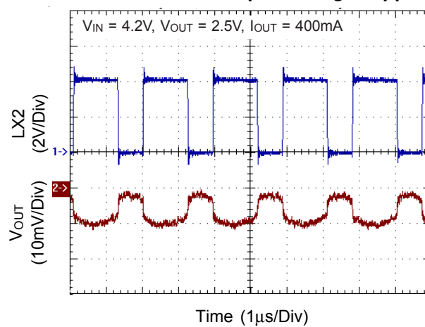
CH2 LX2 and Output Voltage Ripple
