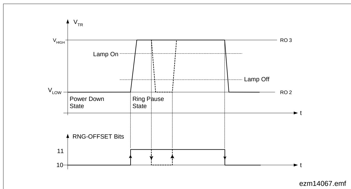
Figure 37 Timing Diagram
