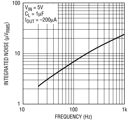
Integrated Noise 10Hz to 1kHz
