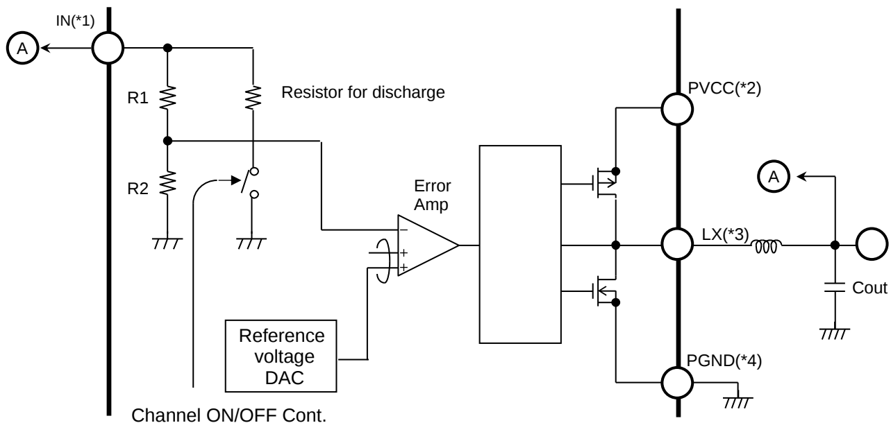
Figure 6. Discharge Function
