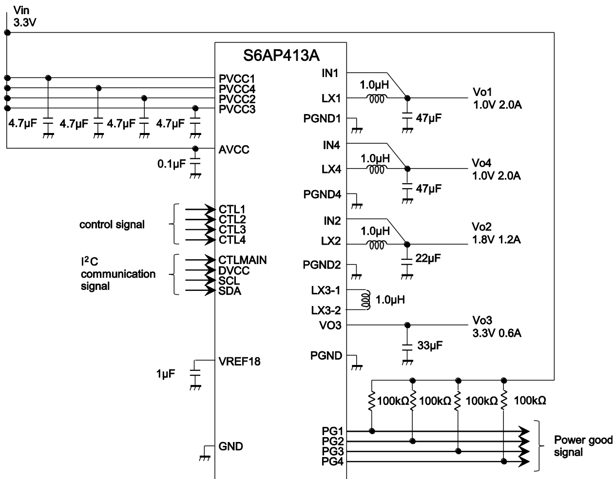
Figure 1. Application Circuit
