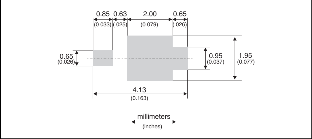
Figure 22. Footprint dimensions
