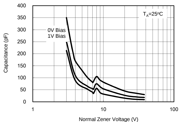
Fig. 6 Typical Capacitance
