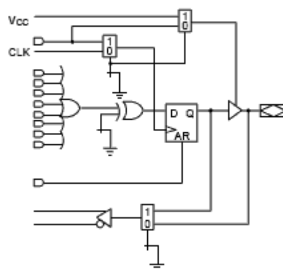
D Register
