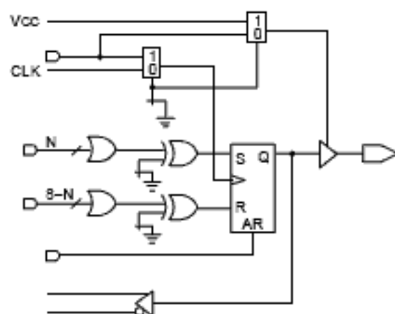
S-R Register
