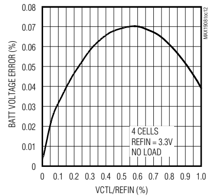
BATT VOLTAGE ERROR vs. VCTL
