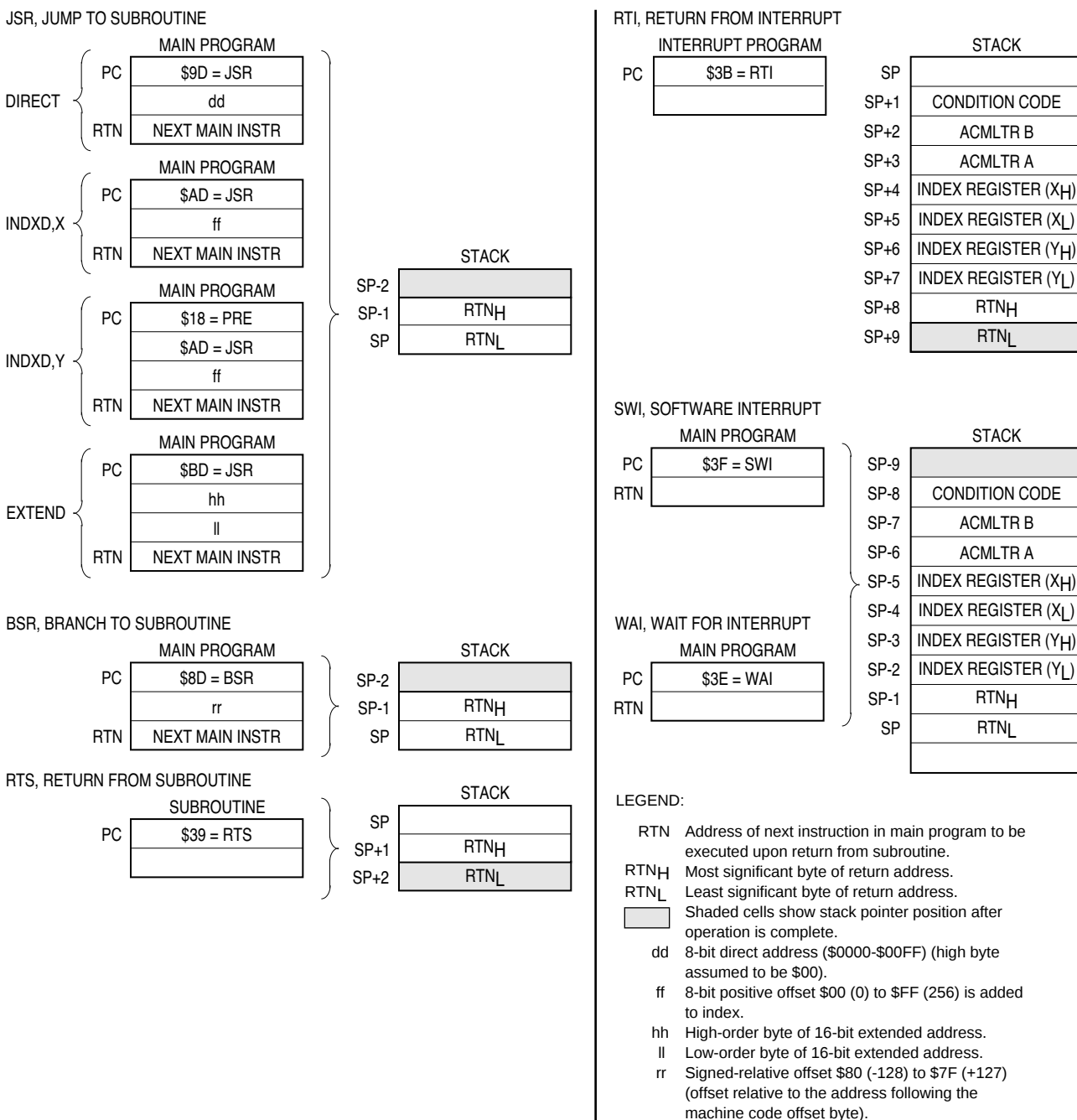
Figure 3-2 Stacking Operations
