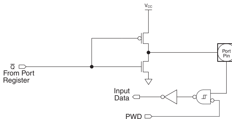
Figure 12-5. Push-pull Output
