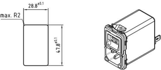
Panel cutout:
