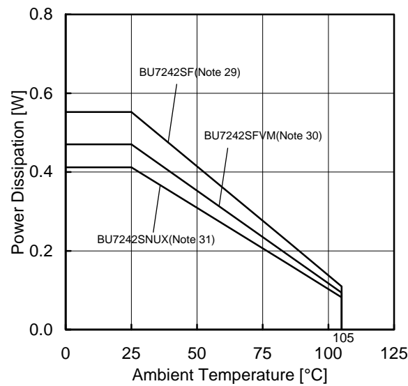
(f)BU7242SF/SFVM/SNUX
