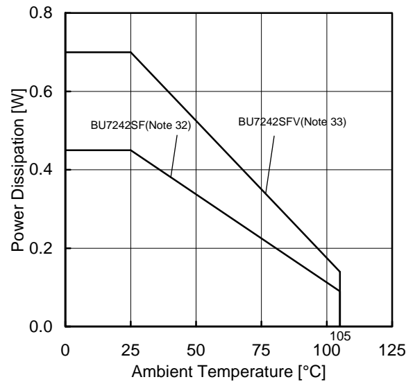
(h)BU7244SF/SFV
