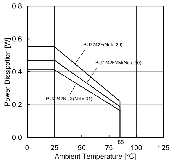
(e)BU7242F/FVM/NUX
