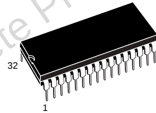
PDIP32 (B)
