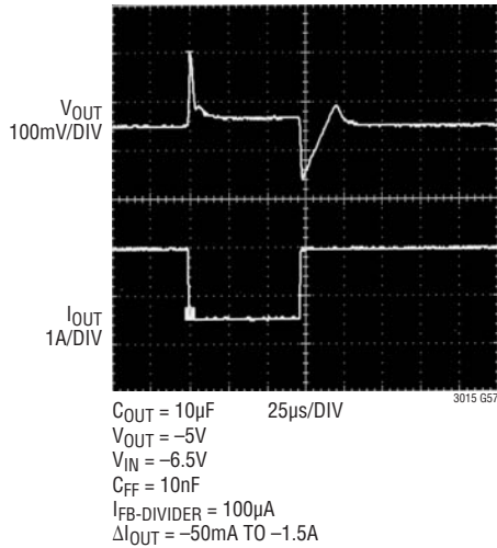
LT3015 Transient Response, C_{FF} = 10\text{nF} , C_{OUT} = 10\mu\text{F}
