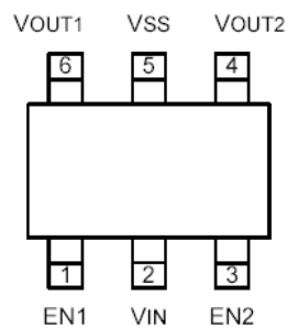
SOT-26 (TOP VIEW)
