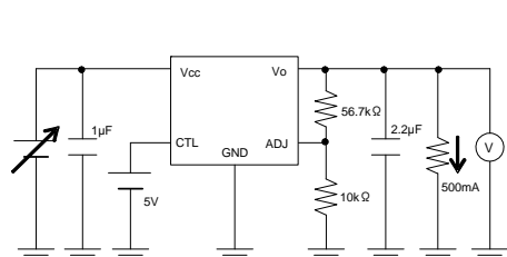
Measurement Circuit of Fig.4
