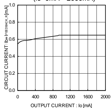
Fig.9 Circuit Current ( I_{\text{FEEDBACK\_R}} \doteq 75\mu\text{A} )
