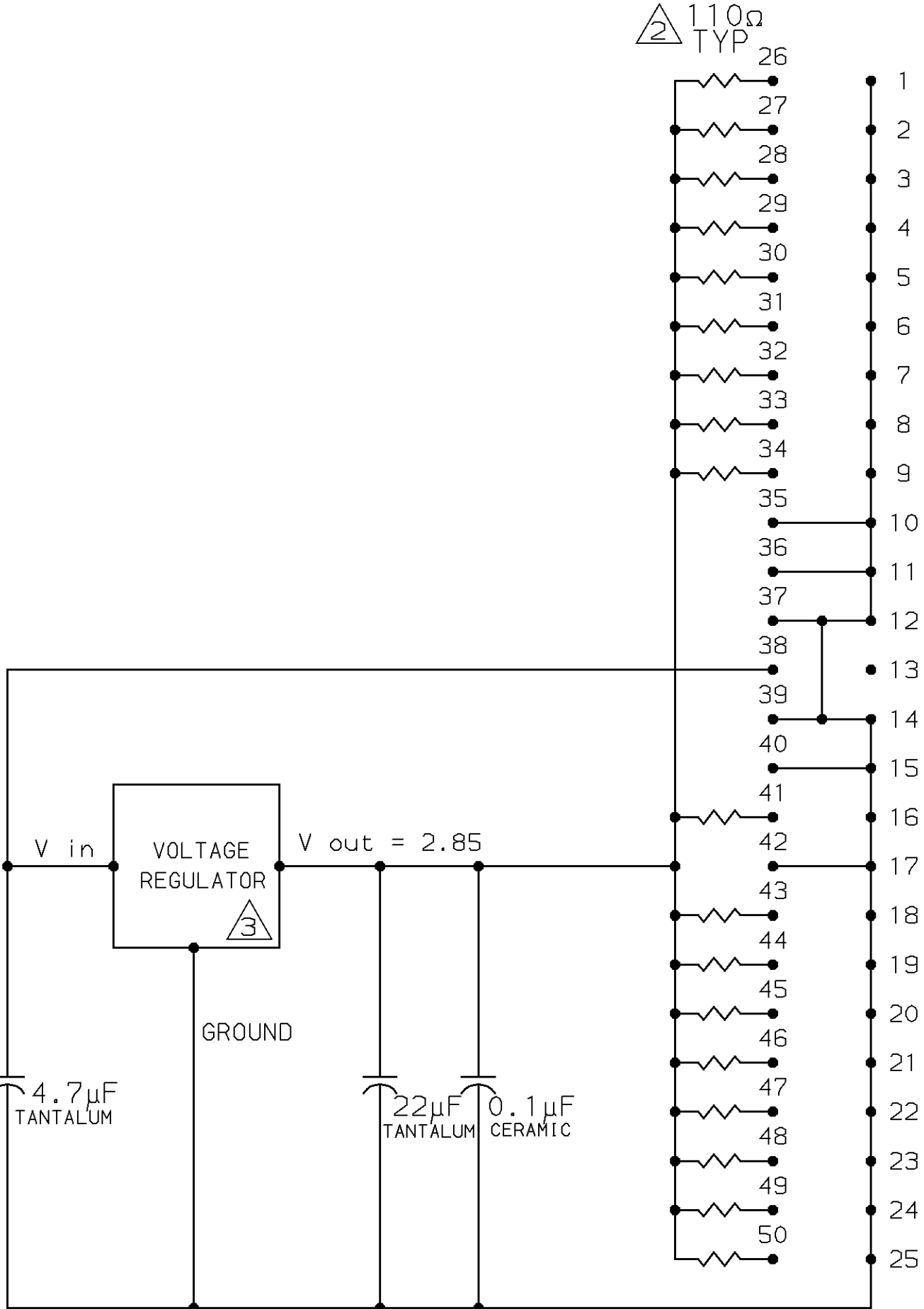
ACTIVE SCHEMATIC
