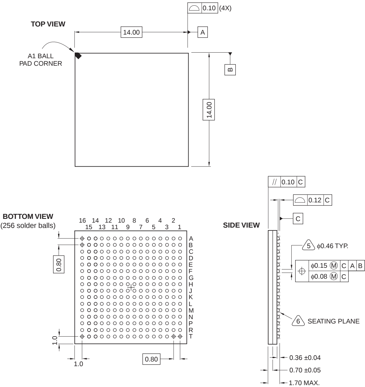
Figure 28. 256-Ball CABGA Package Specification
