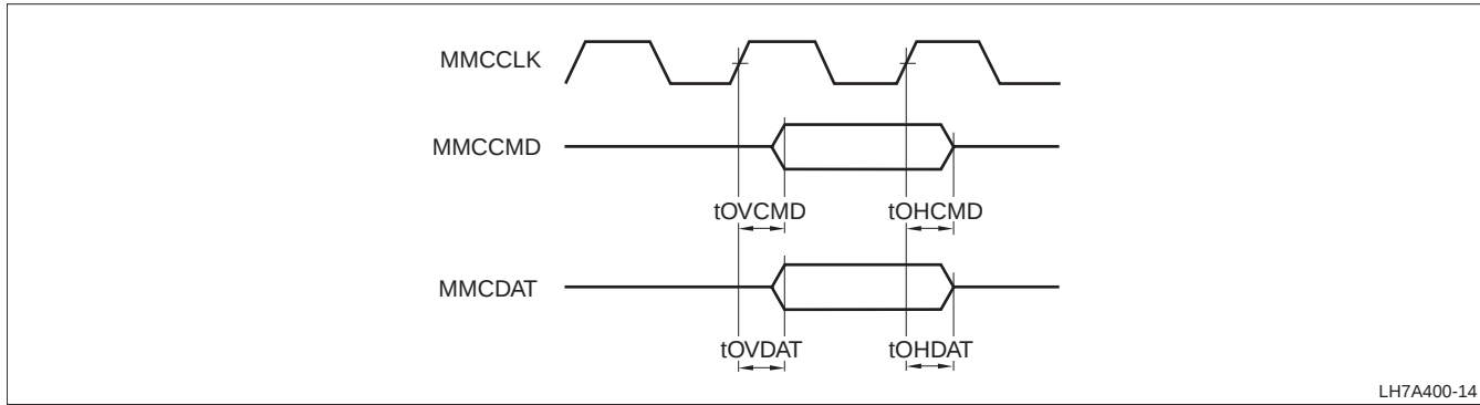
Figure 16. MMC Command/Data Write
