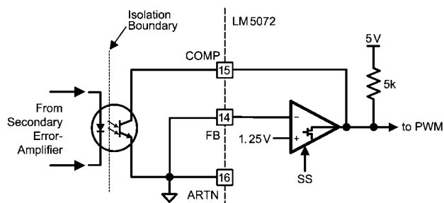
FIGURE 14. The Internal Error Amplifier – Bypassed in Isolated Output Applications
