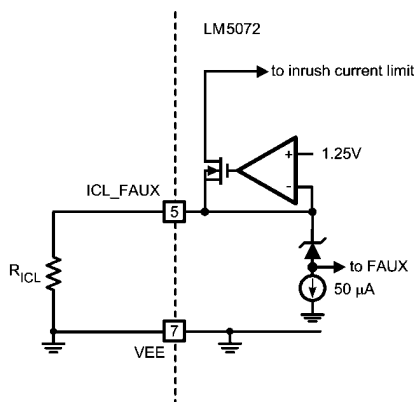
FIGURE 7. Input Inrush Limit Programming via R_{ICL}
