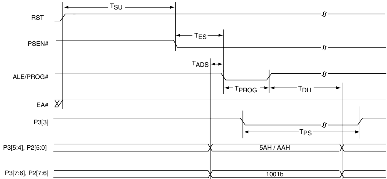
FIGURE 13-22: Prog-SC0 / Prog-SC1
