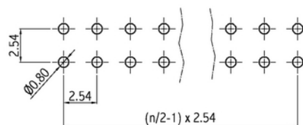
PCB Layouts
