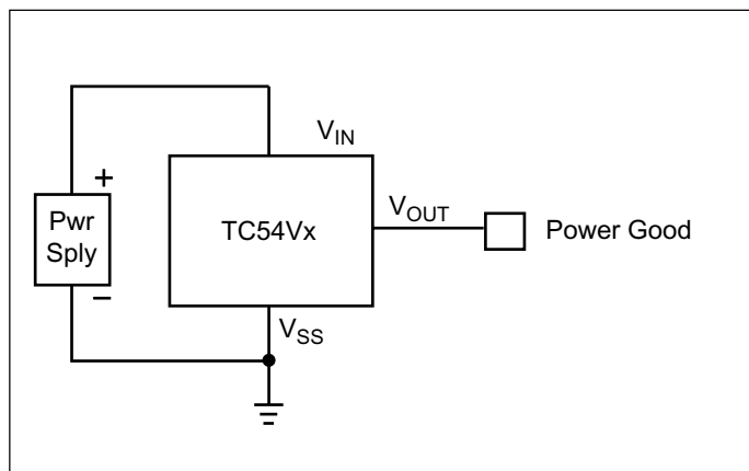
Figure 6: Power good monitor.
