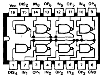
C5 DM8096N Hex Inverter (Tri-state)
