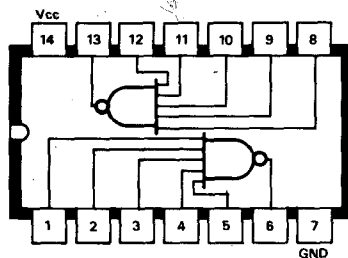
C3 DM8092N Dual 5-input NAND gate
