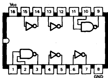
C1 DM8090N NAND Hex Inverter
