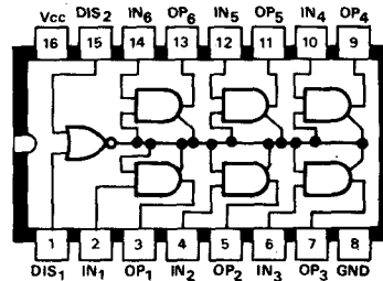
C6 DM8097N Hex buffer 4-2 (Tri-state)
