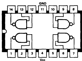
C2 DM8091N Quad 2-input NAND buffer
