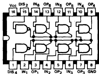
C4 DM8095N Hex buffer (Tri-state)
