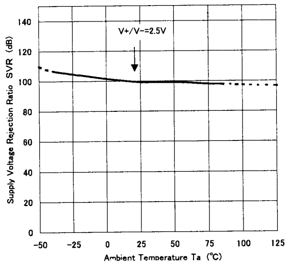
NJM13403 Supply Voltage Rejection Ratio vs.
