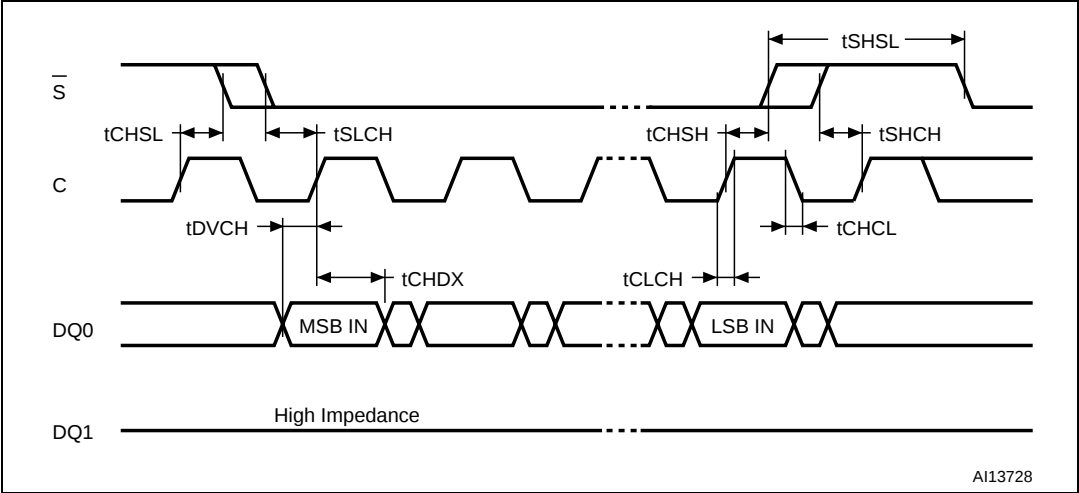
Figure 108. Serial input timing
