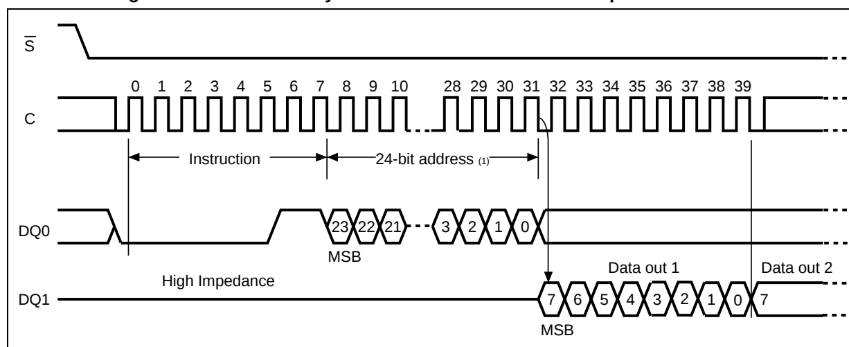
Figure 11. Read Data Bytes instruction and data-out sequence
