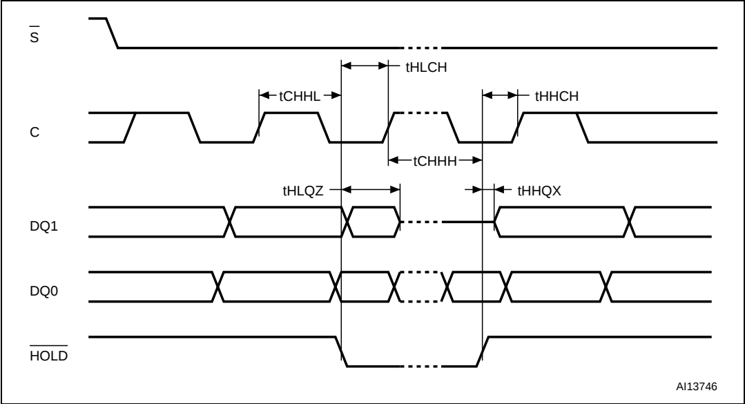
Figure 110. Hold timing
