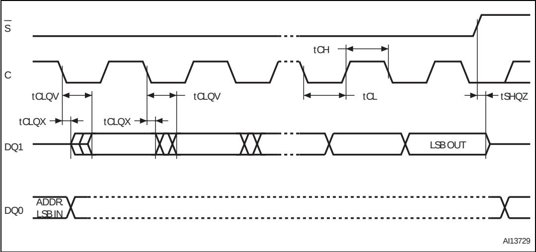
Figure 111. Output timing
