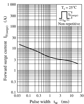
I_{F(\text{surge})} - t_w
