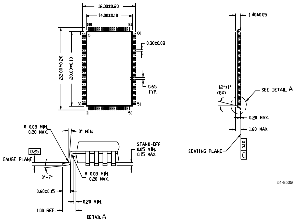
100-Pin Thin Plastic Quad Flatpack (14 x 20 x 1.4 mm) A101
