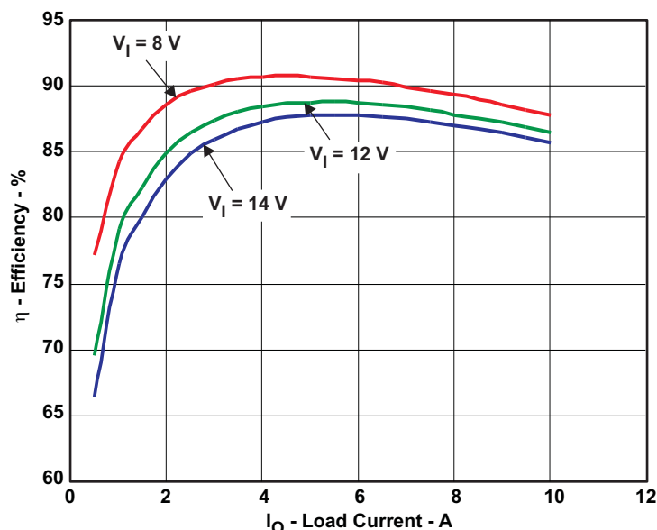
Figure 5. TPS40192EVM-525 Efficiency vs Load Current, V_{in} = 8\text{ V} - 14\text{ V} , V_{out} = 1.8\text{ V} , I_{out} = 0\text{ A} - 10\text{ A}
