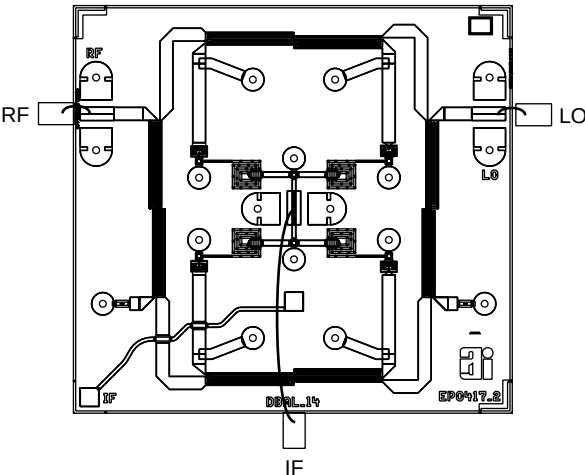
Single IF bond configuration.
