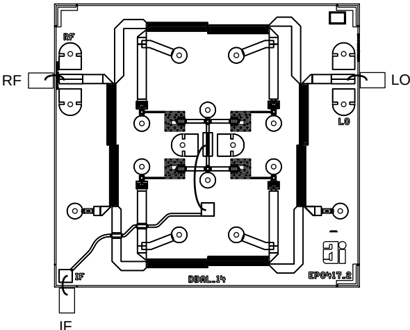
Requires two IF bonds. LO to IF isolation is degraded by 7 dB for this configuration.
