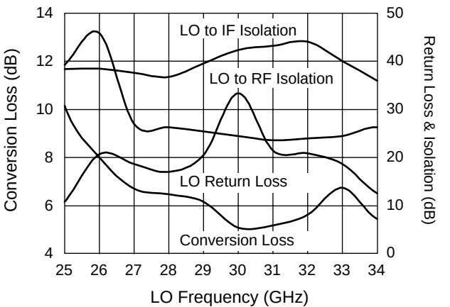
Performance vs. LO Frequency
