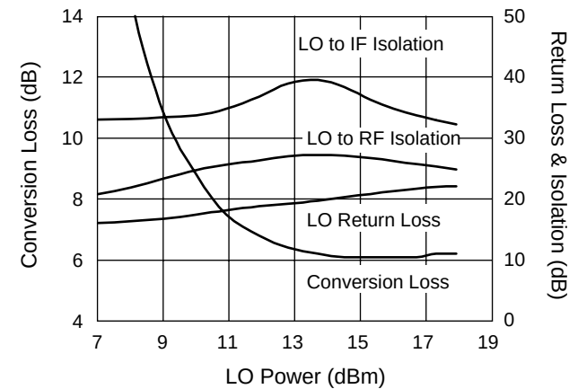
Performance vs. LO Power
