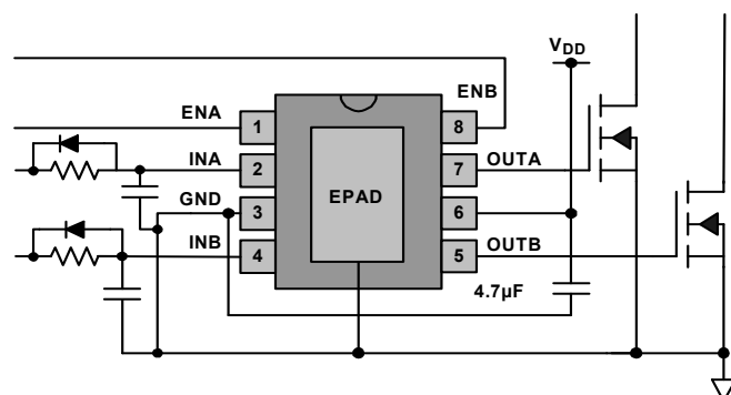
Figure 1. Typical Application
