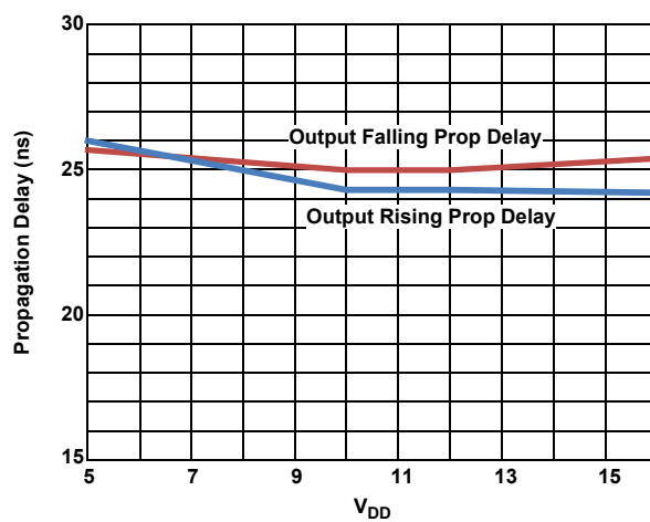
Figure 18. Propagation Delay vs V_{DD}
