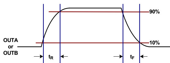
Figure 5. Rise/Fall Times
