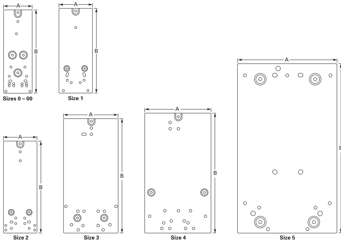
Figure 33-33. Approximate Dimensions
