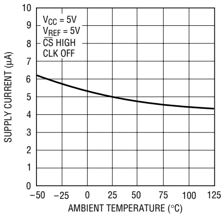
LTC1297 Supply Current (Power Shutdown) vs Temperature
