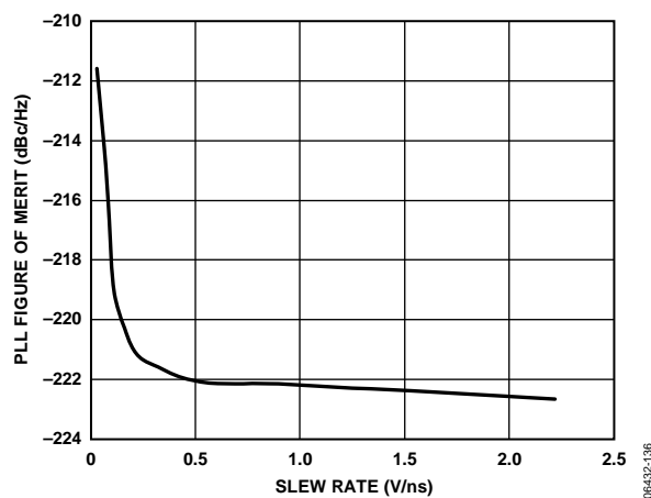
Figure 10. PLL Figure of Merit (FOM) vs. Slew Rate at \overline{\text{REFIN}}/\text{REFIN}
