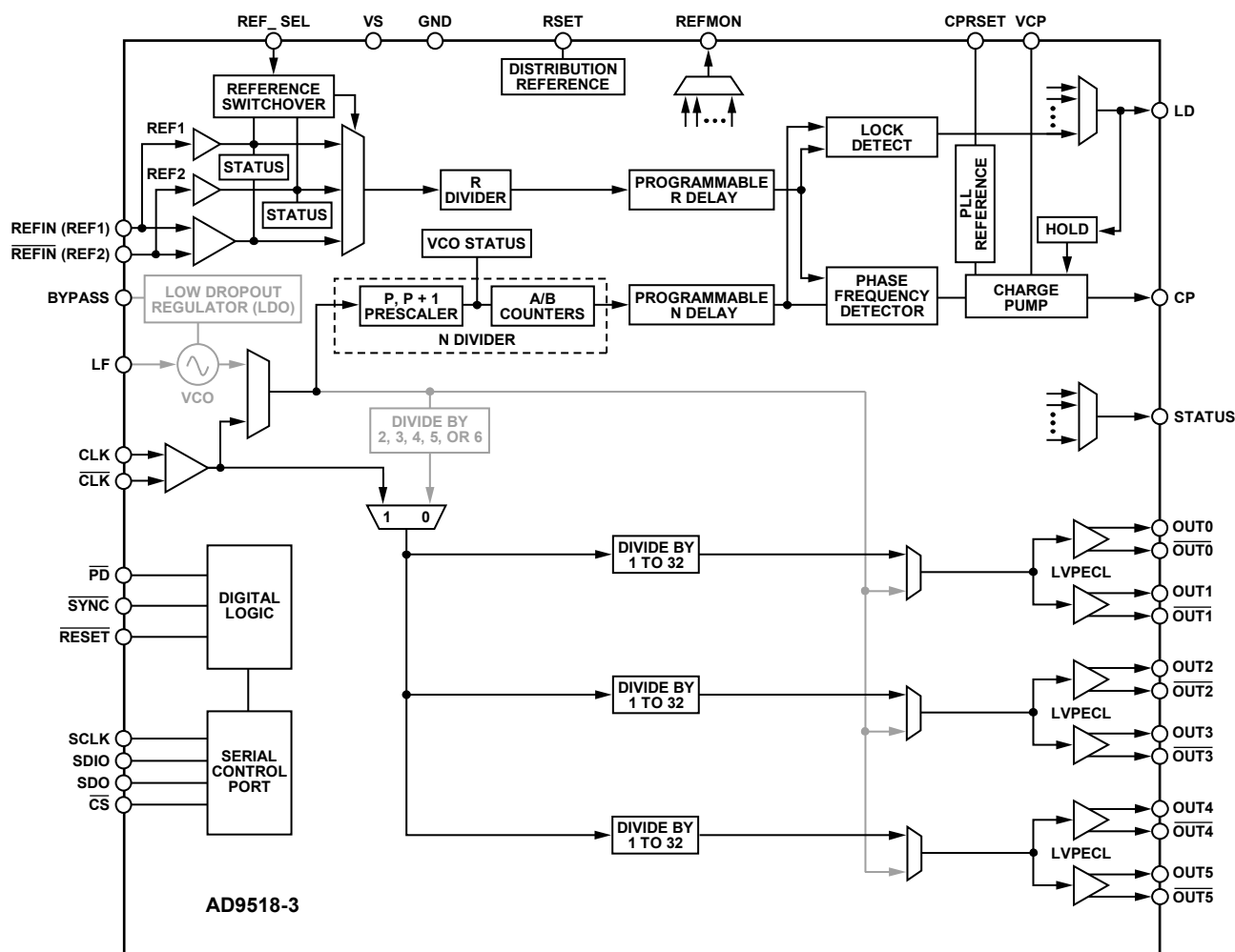
Figure 30. Clock Distribution of External VCO < 1600 MHz
