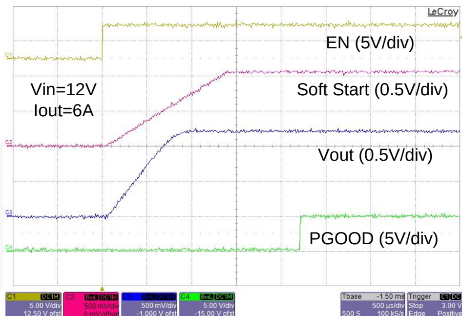
Figure 5. Typical FAN2306 Startup Waveforms
