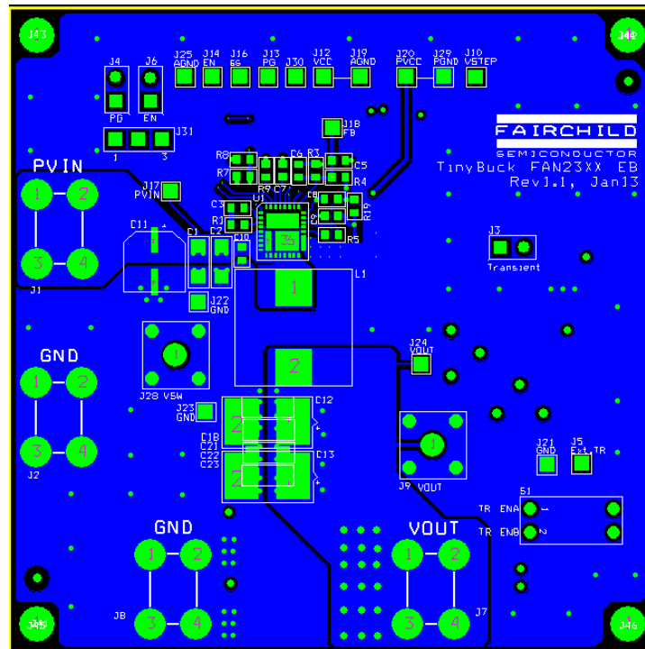
Figure 7. Top Side
