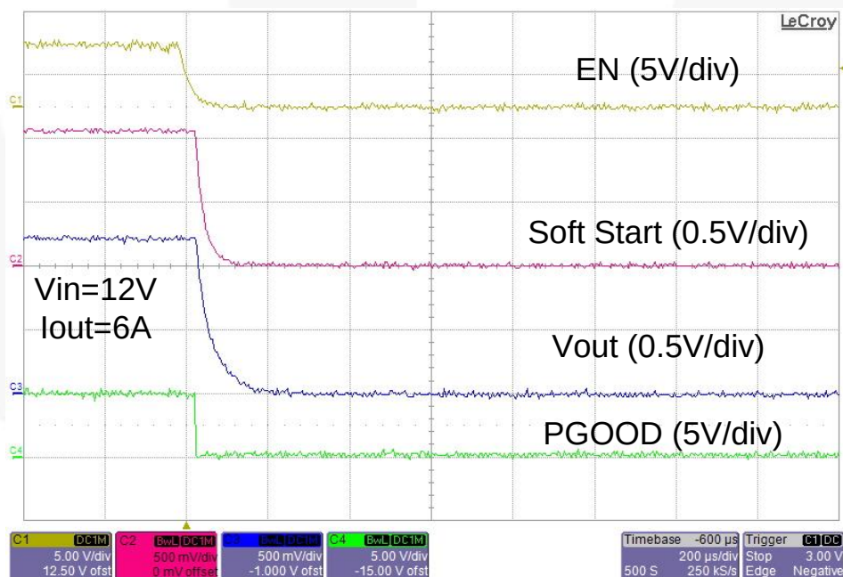
Figure 6. Typical FAN2306 Shutdown Waveforms
