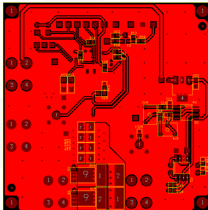
Figure 8. Bottom Side
