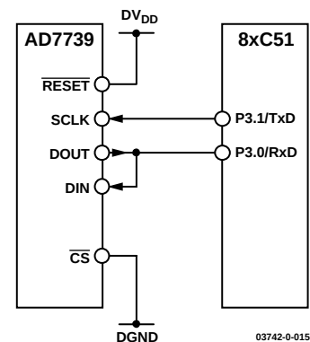
Figure 14. AD7739 to Host Device Interface, 2-Wire Configuration
