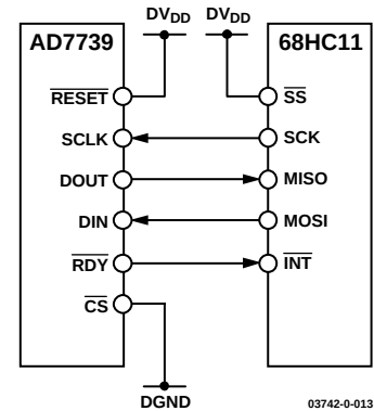
Figure 12. AD7739 to Host Device Interface, SPI
